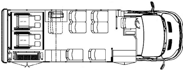
Side Lift - 8 Passenger and 2 Wheelchair
