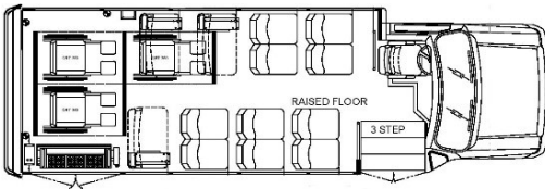
Side Lift - 12 Passenger and 3 Wheelchair
