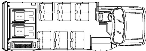
Side Lift - 12 Passenger and 2 Wheelchair
