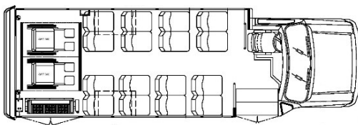
Side Lift - 13 Passenger and 2 Wheelchair
