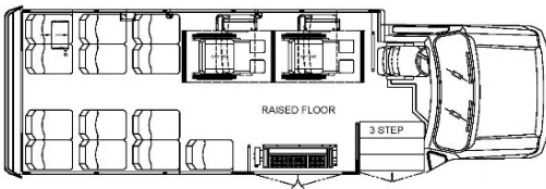
Side Front Lift - 13 Passenger and 2 Wheelchair
