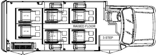
Side Lift - up to 8 Passenger and 6 Wheelchair
