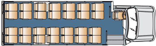
28 Passenger Plus Driver
